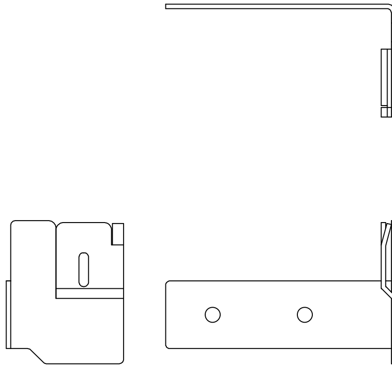
X-501a Tee Bar Connector Clip
