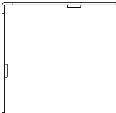
X-CC1 Upstand, Internal Corner Clip supplied c/w 2 No. fixing screws
