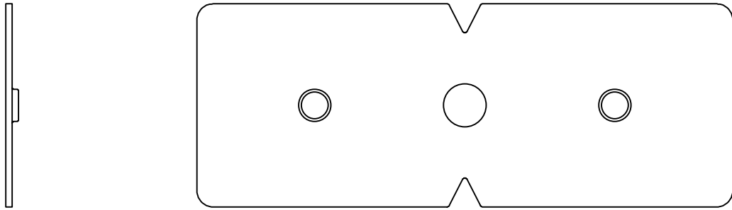
X-SP1 Upstand, Straight Splice Clip supplied c/w 2 No. fixing screws
