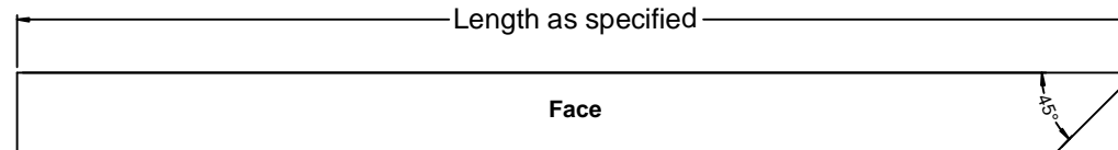
MOE/RH Mitred One End - Right Hand
